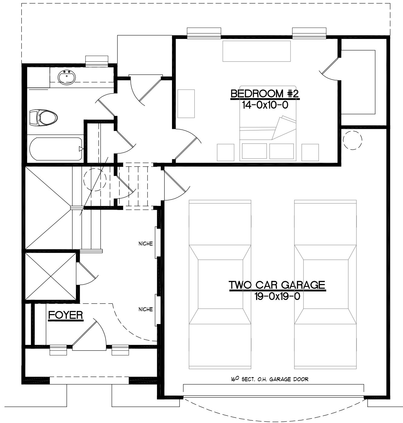
First Floor Layout - 535 sqft.
