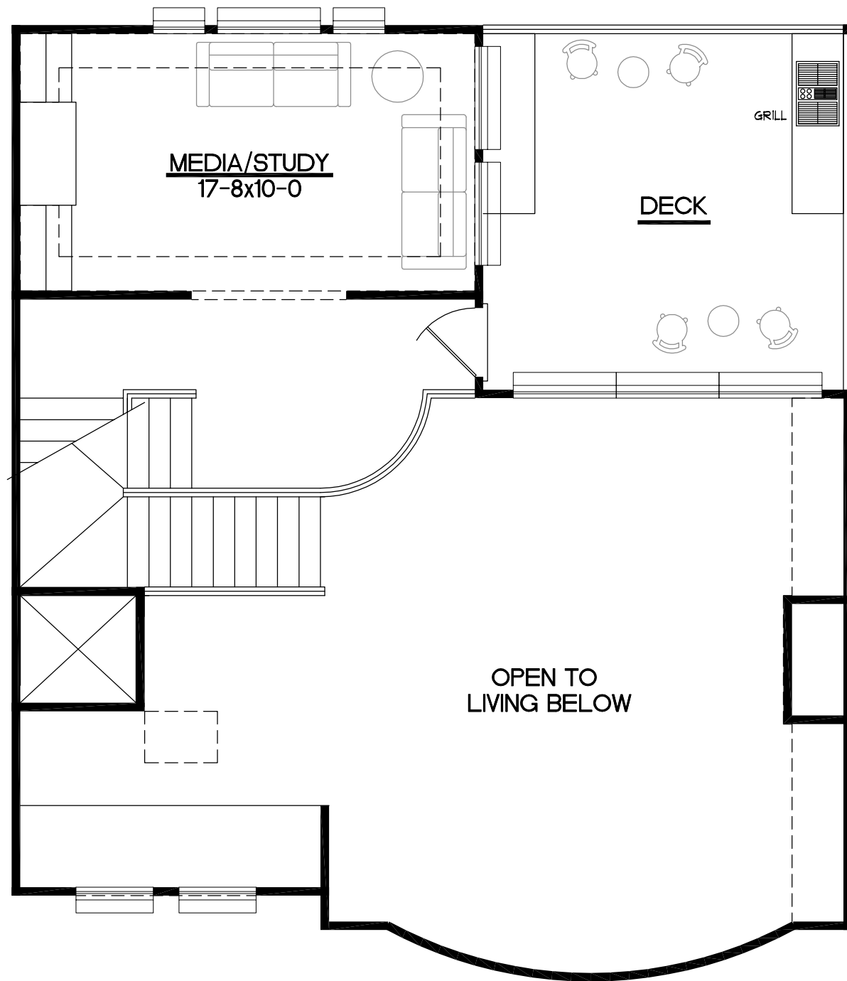
Third Floor Layout - 298 sqft.
